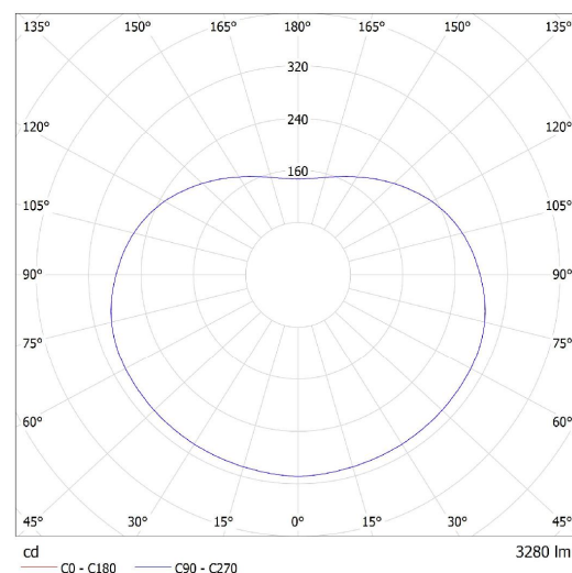
Lucis ZKS.L2.400.X POLARIS ZKS LED / LDC (Polar)
